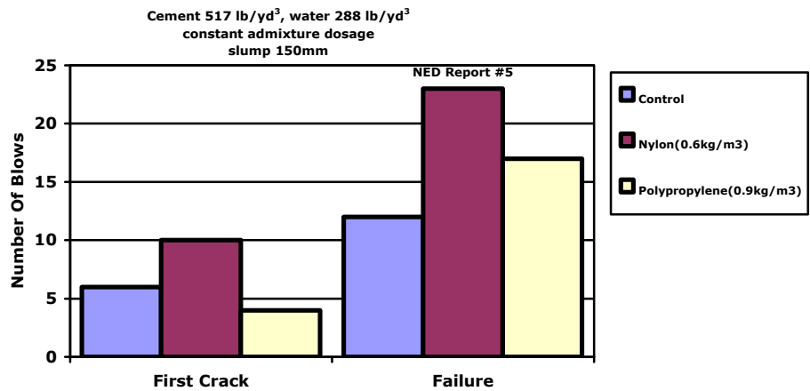
Figure 2-Impact Resistance
